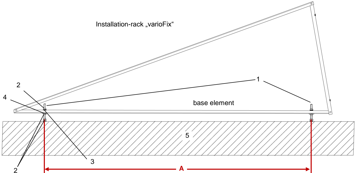
Installation-rack with concrete element (5) and studding (1) on a robust sustainable basement / ground
