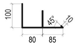
Detail side sheet
