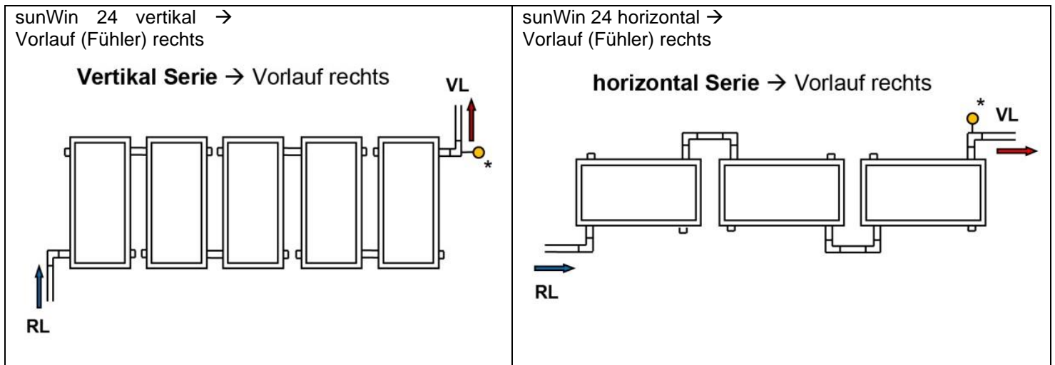
Detail A
